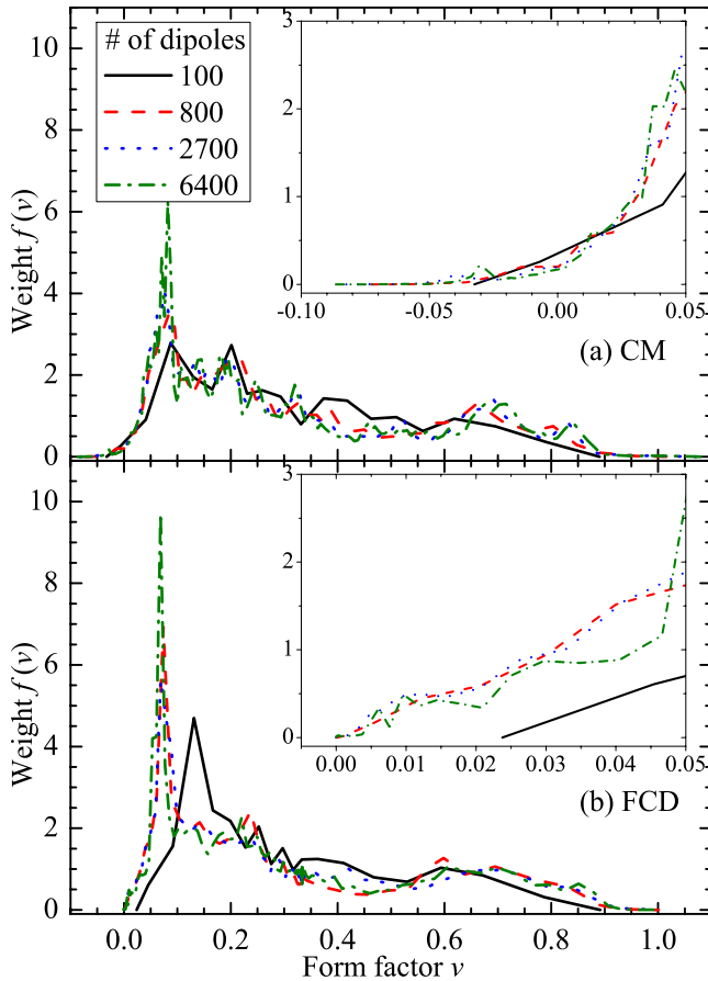
FIG. 8. (Color online) Form-factor distributions for GRF2 particle, computed using the CM (a) and the FCD (b). Results are obtained by smoothing (see text) from sets \{v_n, f_n\} obtained for several levels of discretization. Insets show detailed behavior near zero values of v .
